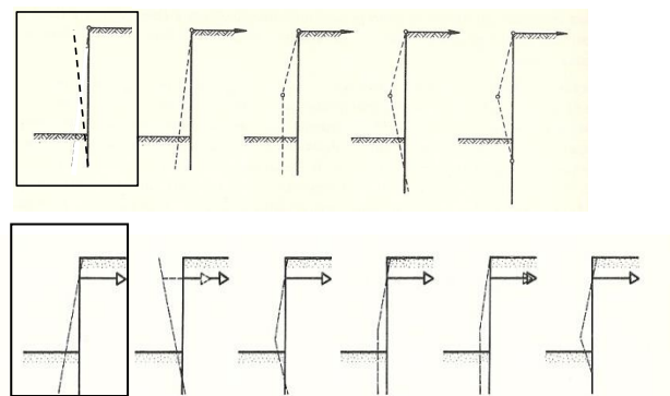
Figure 2 A wall in failure composed of one or more rigid segments connected by yield hinges in failure. This paper deals with the two left hand cases
