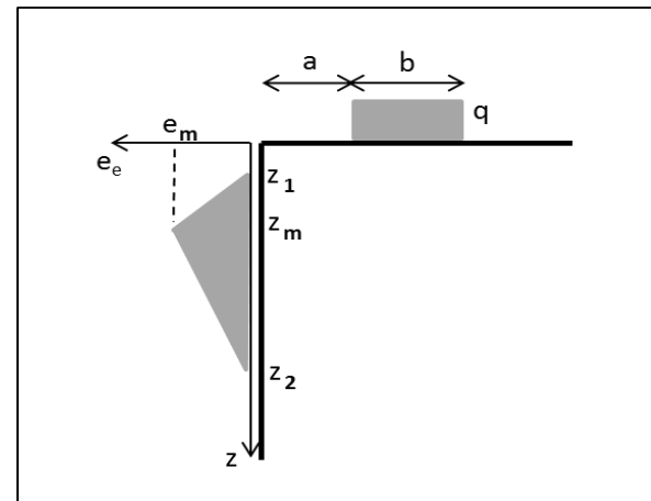
Figure 7 Triangular approximated distribution for the Boussinesq's solution where the strip footing is assumed as a line load ( z_1 = 0 ; z_m = 0.4(a+0.5b) ; z_2 = 2.5(a+0.5b) ; e_m = 0.45qb/(a+0.5b) \cdot p ).
