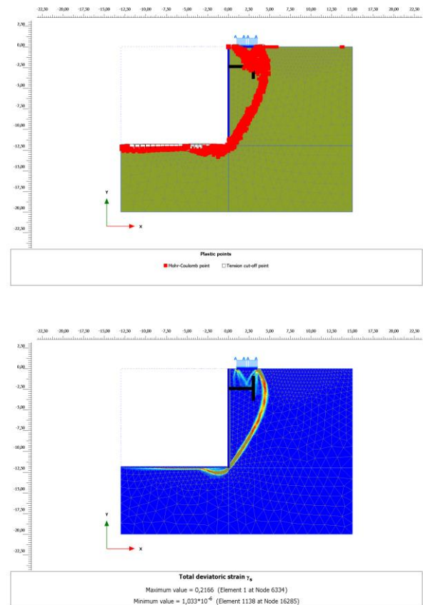
Figure 9 Anchored Wall, 2D FE plain strain results (plastic points & deviatoric strains), \phi=30^\circ , a=1.0 m, b=2.5 m, or a/b=0.4 , p=125 kPa.
