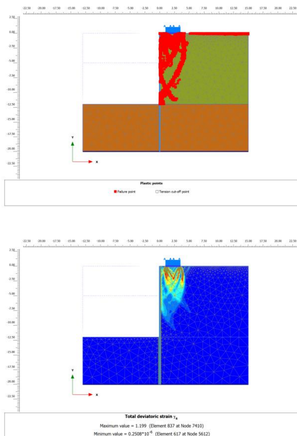
Figure 8 Free Wall, 2D FE plain strain results (plastic points & deviatoric strains), \phi=30^\circ , a=1.0 m, b=2.5 m, or a/b=0.4 , p=125 kPa.
