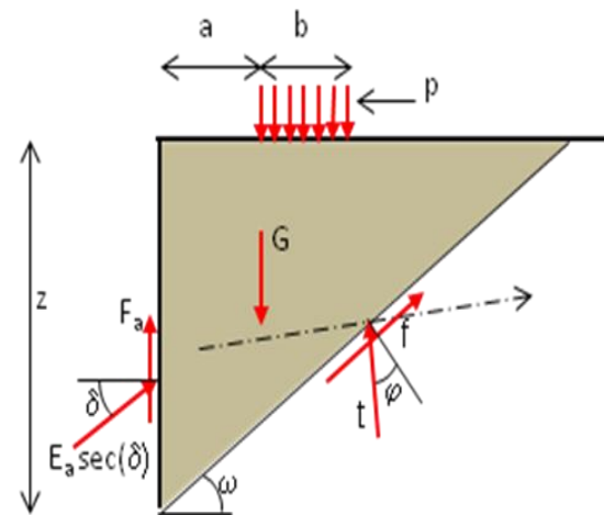
Figure 3 Coulomb's Method
